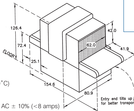
Dimensions are in centimeters Note: Non-marring casters
